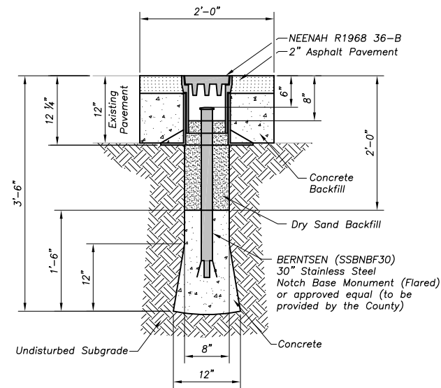
MONUMENT AND BOX WITH EXISTING PAVEMENT
