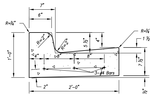
Standard Type "B" Curb
