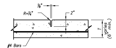
Contraction Joint
